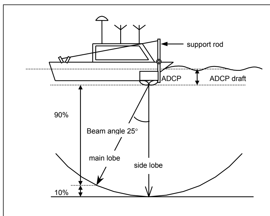
Figure 6.45(c): Relationship between transducer beam angle and thickness of the contaminated layer
