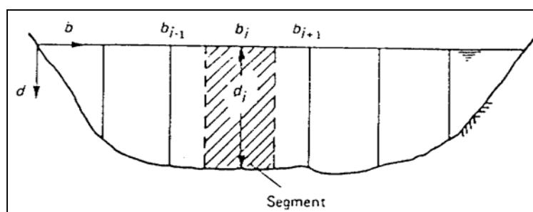
Figure 6.40: Sketch illustrating the computation of discharge using the mid-section method
